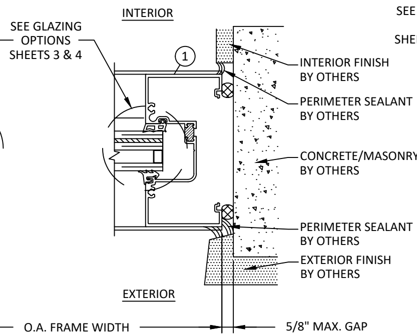
H HORIZONTAL SECTION 11 JAMB - DIRECT TO CONCRETE/MASONRY STANDARD CONFIGURATION
