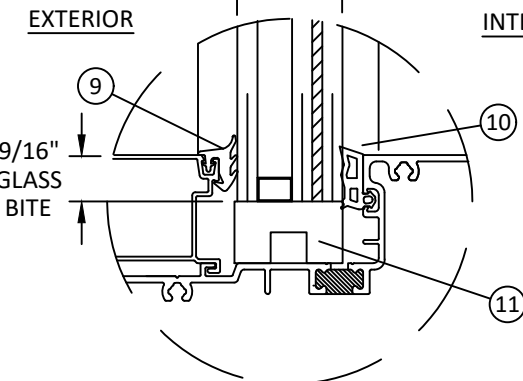
GLAZING DETAIL D (DRY GLAZED)
