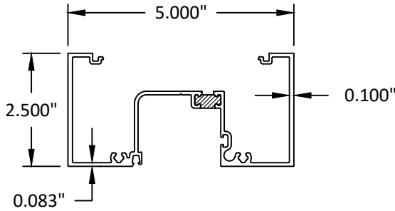
1 HEAD/JAMB/VERTICAL
