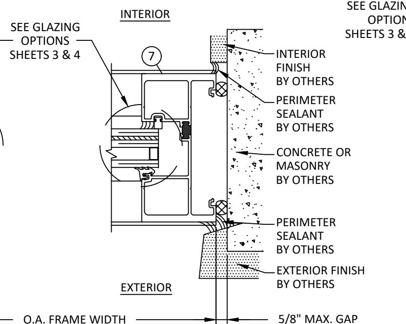
L HORIZONTAL SECTION 11 JAMB - DIRECT TO CONCRETE/MASONRY HEAVY CONFIGURATION
