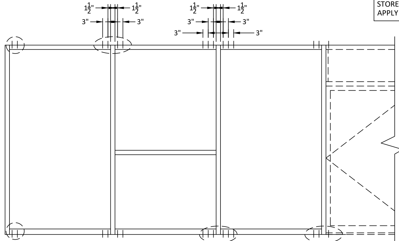
TYPICAL ANCHOR LAYOUT
