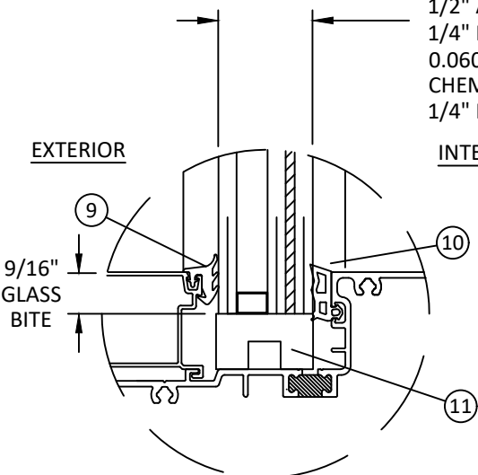
GLAZING DETAIL B (DRY GLAZED)
